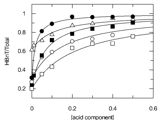
Figure 3a. Formation of HBnT versus fragmentation: pH = pK a (○ bis-tris pH 6.7, • pyridine pH 5.4, (□) (2,2,2)-trifluoroethylamine pH 5.7, phosphate pH 6.5, and Δ acetate pH 4.6).
