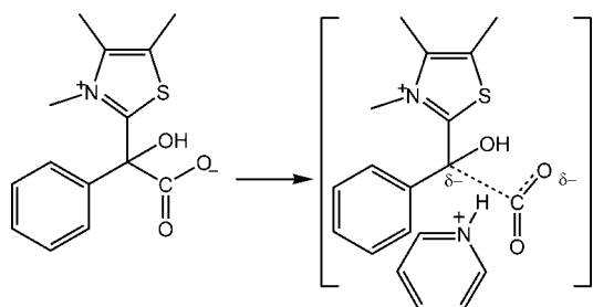
Figure 3. Buffer catalyzed decarboxylation of MT.
