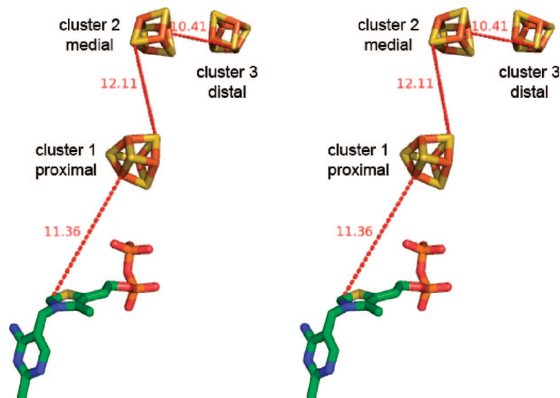
Figure 7. Relative orientation of cofactors in PFOR in stereoview.
