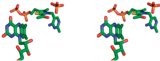
Figure 12. X-ray structure of FAD, HETDP enamine, and phosphate in POX prior to electron transfer. 76
