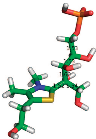
Figure 19. Partial DFT optimization of the X5P-TDP adduct (here a simplified thiazolium model) suggests a selective weakening of the scissile C2–C3 bond in the conformation of the intermediate formed at the active site.
